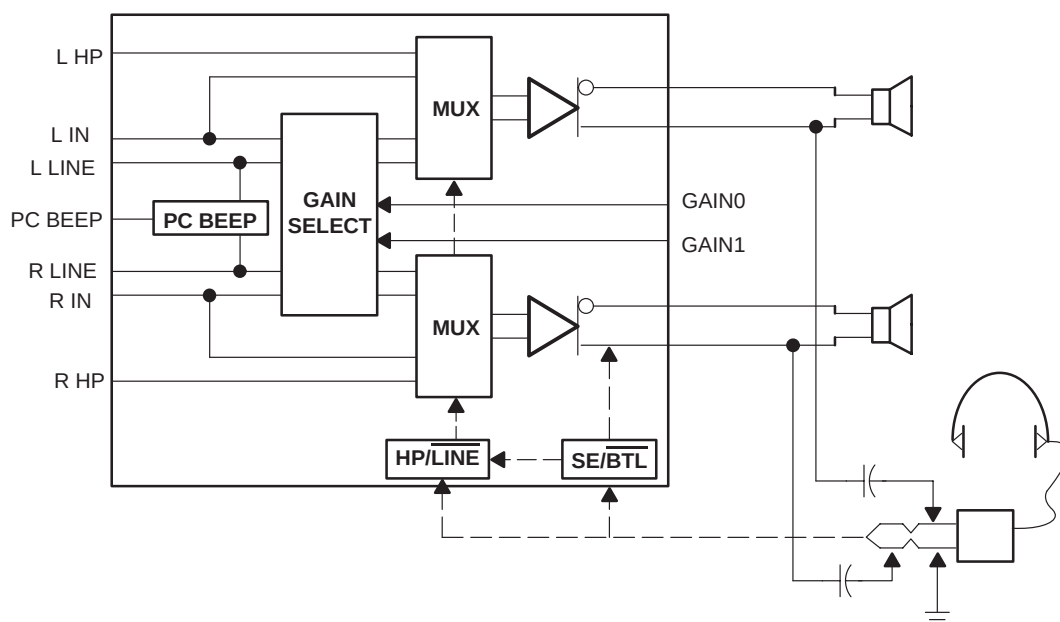
Figure 3–4. TPA0212 Amplifier IC
